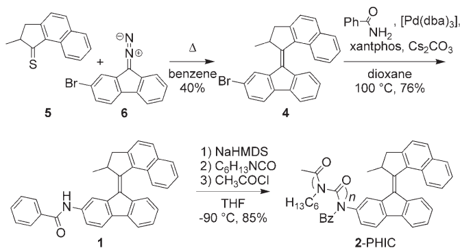
Scheme 1. Synthesis of benzamide-functionalized motor 1 and formation of 2-PHIC ((2′ S )-( M )- trans - 2-PHIC : M_w = 19\,700 ; (2′ S )-( M )- cis - 2-PHIC : M_w = 28\,700 ). Bz = benzoyl, dba = trans,trans -dibenzylideneacetone, HMDS = hexamethyldisilazide, xantphos = 4,5-bis(diphenylphosphino)-9,9-dimethylxanthene.
