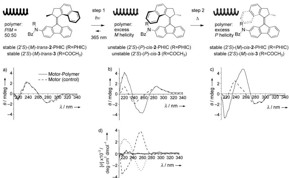
Figure 3. CD spectra (Et 2 O, -20^\circ\text{C} ) of a) (2′ S )-( M )- trans - 2-PHIC (15.0 mg L -1 ; solid line) and (2′ S )-( M )- trans - 3 (1.11 μM; dotted line); b) step 1: the PSS mixture with (2′ S )-( M )- trans - 2-PHIC and (2′ S )-( P )- cis - 2-PHIC (solid line), and the PSS mixture with (2′ S )-( M )- trans - 3 and (2′ S )-( P )- cis - 3 (dotted line) after irradiation (365 nm); c) step 2: the mixture of (2′ S )-( M )- trans - 2-PHIC and (2′ S )-( M )- cis - 2-PHIC (solid line) and the mixture of (2′ S )-( M )- trans - 3 and (2′ S )-( M )- cis - 3 (dotted line) after irradiation and storage in the dark at 20^\circ\text{C} for 30 min. d) Molar ellipticity spectra of the polymer backbone (CD difference spectra: polymer 2 –acetylated motor 3 ) for the stable (2′ S )-( M )- trans isomer of the motor (solid line), after irradiation (dotted line), and after irradiation and storage in the dark at 20^\circ\text{C} (dashed line).
